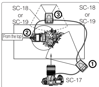
Multiple flash shooting (using 3 flash units)
